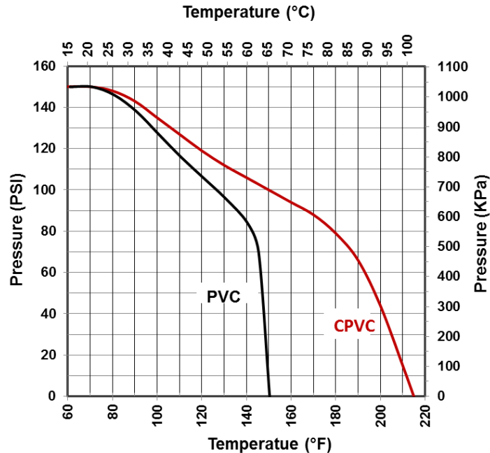
Graph 1: Operating Pressures of PVC and CPVC Materials at Elevated Temperatures.
