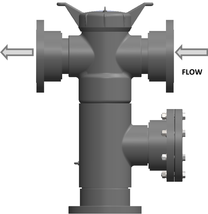
Fig. 2: Straight Flow Connection
