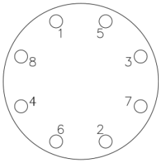
Fig. 4: Bolt Tightening Sequence
