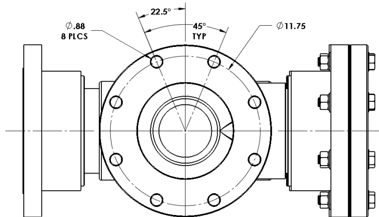
Figure 1: SB Series 6" & 8" Base, Bottom View
