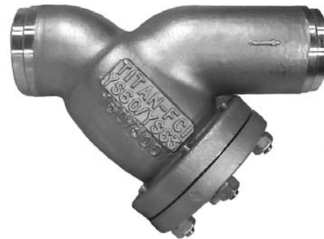
Figure 6: WYE Strainer ~ Butt-Weld Ends
